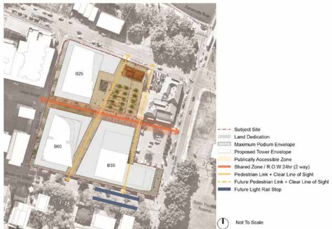
Figure 4.3.3.7.57 Master plan diagram for 142-154 Macquarie Street, Parramatta
