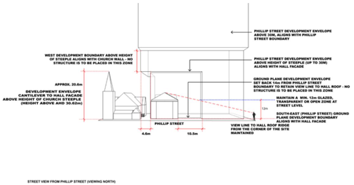
Figure 4.3.3.7.30 Maximum building envelope – Ground plane details, view from Phillip Street NTS (TKD Architects 2016)
