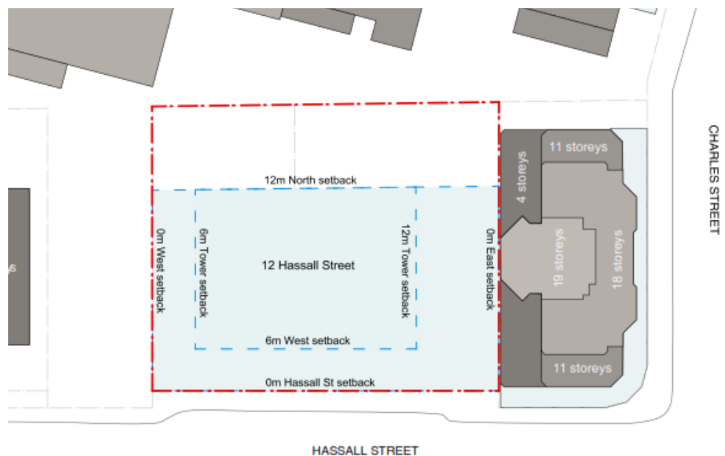
Figure 4.3.3.7.75 Built form – setback and tower separations.
