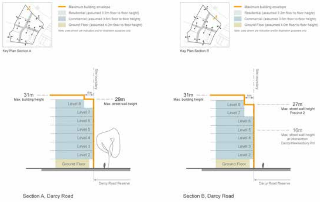
Figure 4.3.4.1.8 Indicative Site Sections
