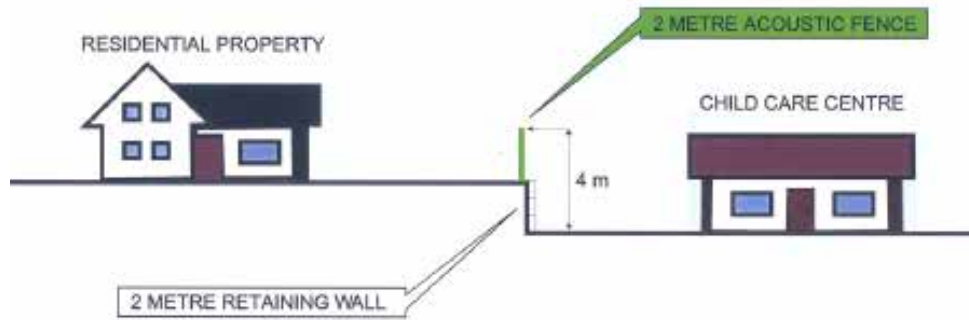
Examples of acoustic barrier designs for sloping sites where an effective height of up to 4 m is required
