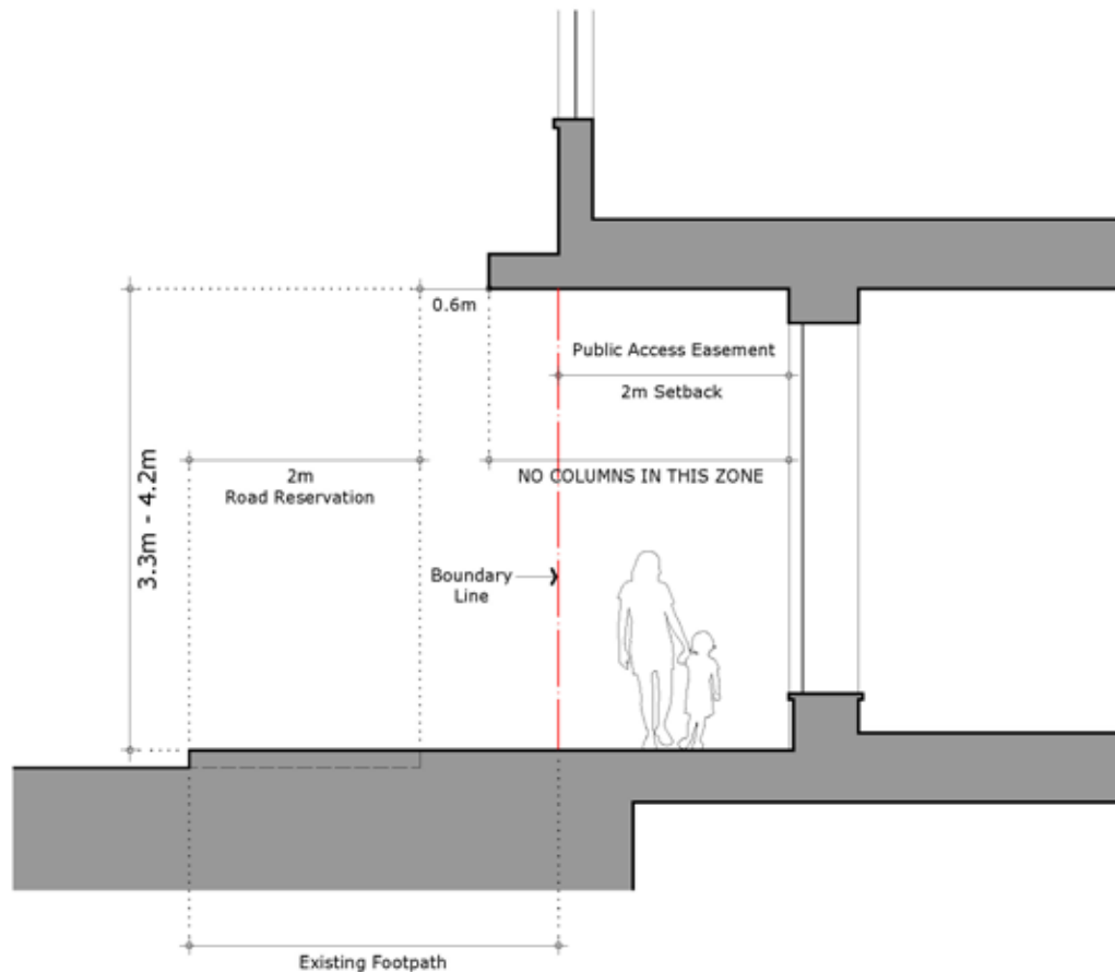
Figure 4.3.3.7.85 Detailed Section through Marsden Street
