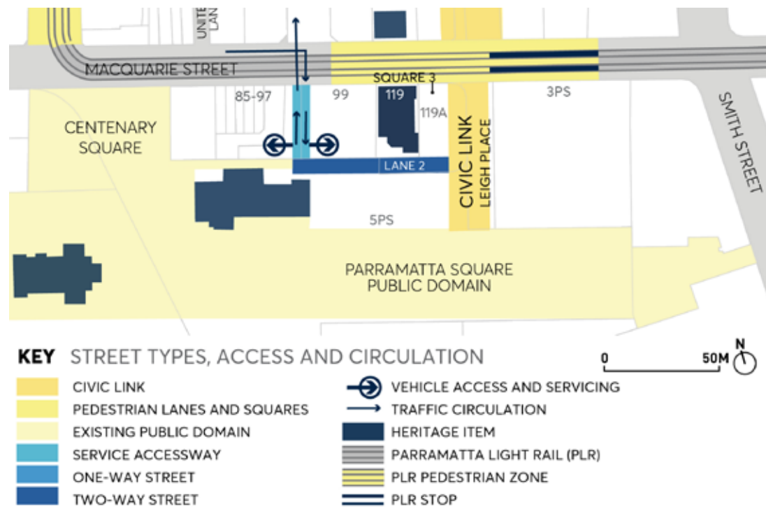
Figure 4.3.3.7.54 Street Types, Access and Circulation
