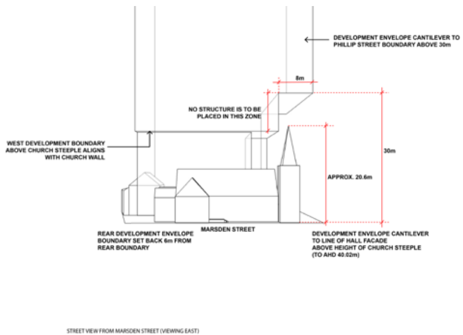
Figure 4.3.3.7.31 Maximum building envelope – Ground plane details, view from Marsden Street NTS (TKD Architects 2016)
