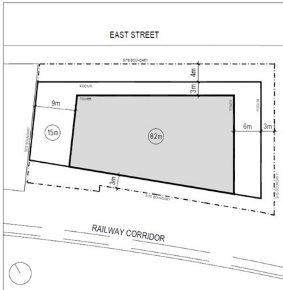
Figure 4.3.7.2.3 Building Height and Setback Control
