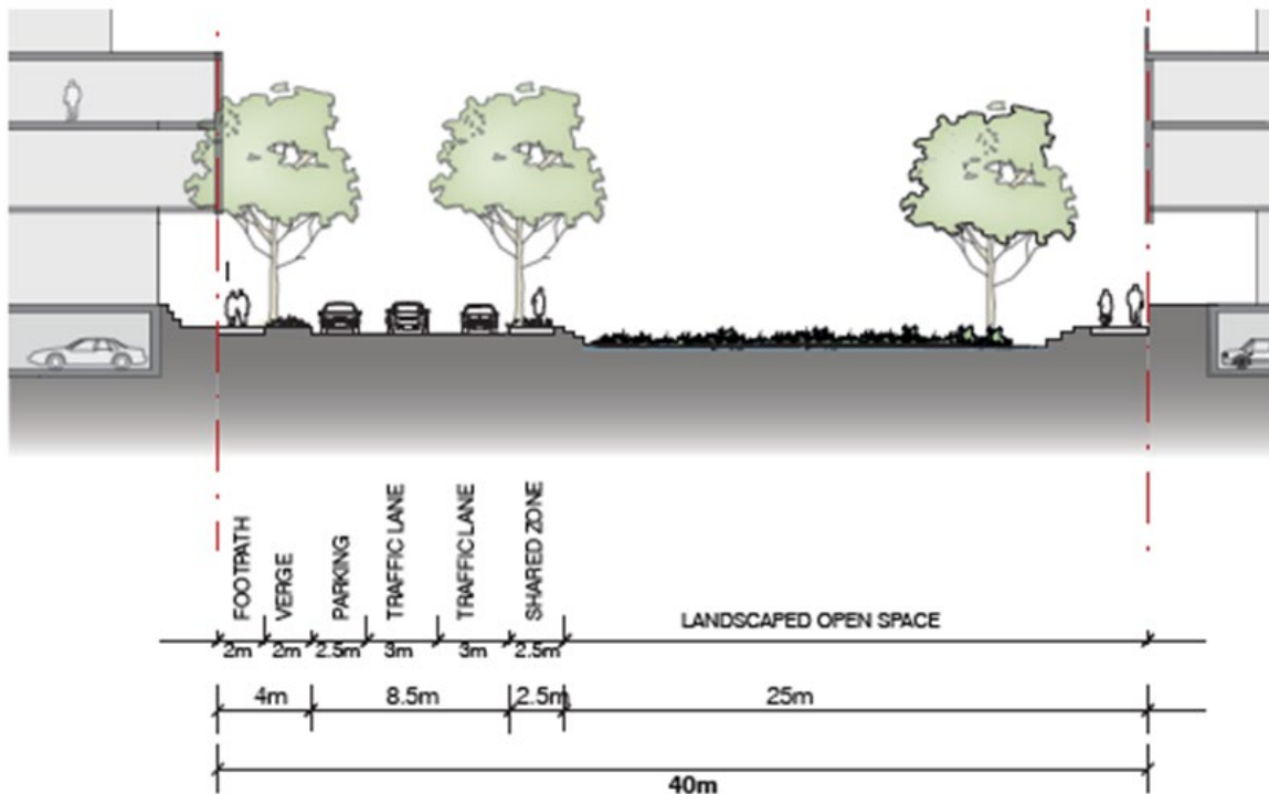
Figure 10: Section AA
