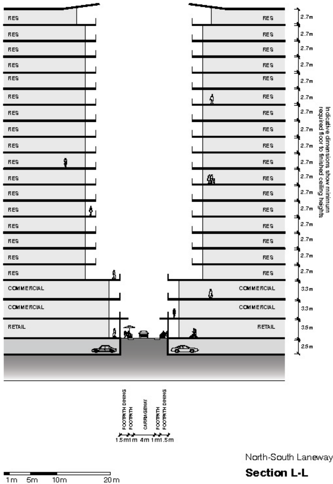
Figure 12: Section L-L
