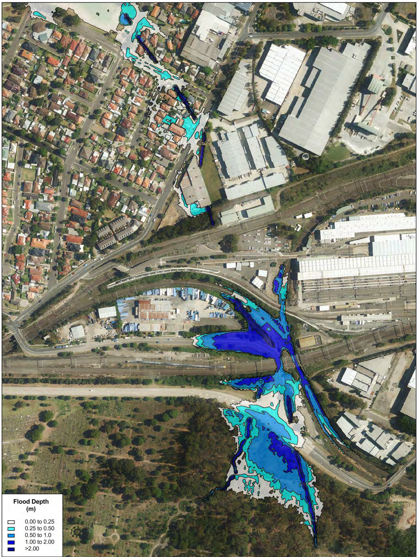
FIGURE B1 Existing Scenario - 5% AEP Flood Depths
