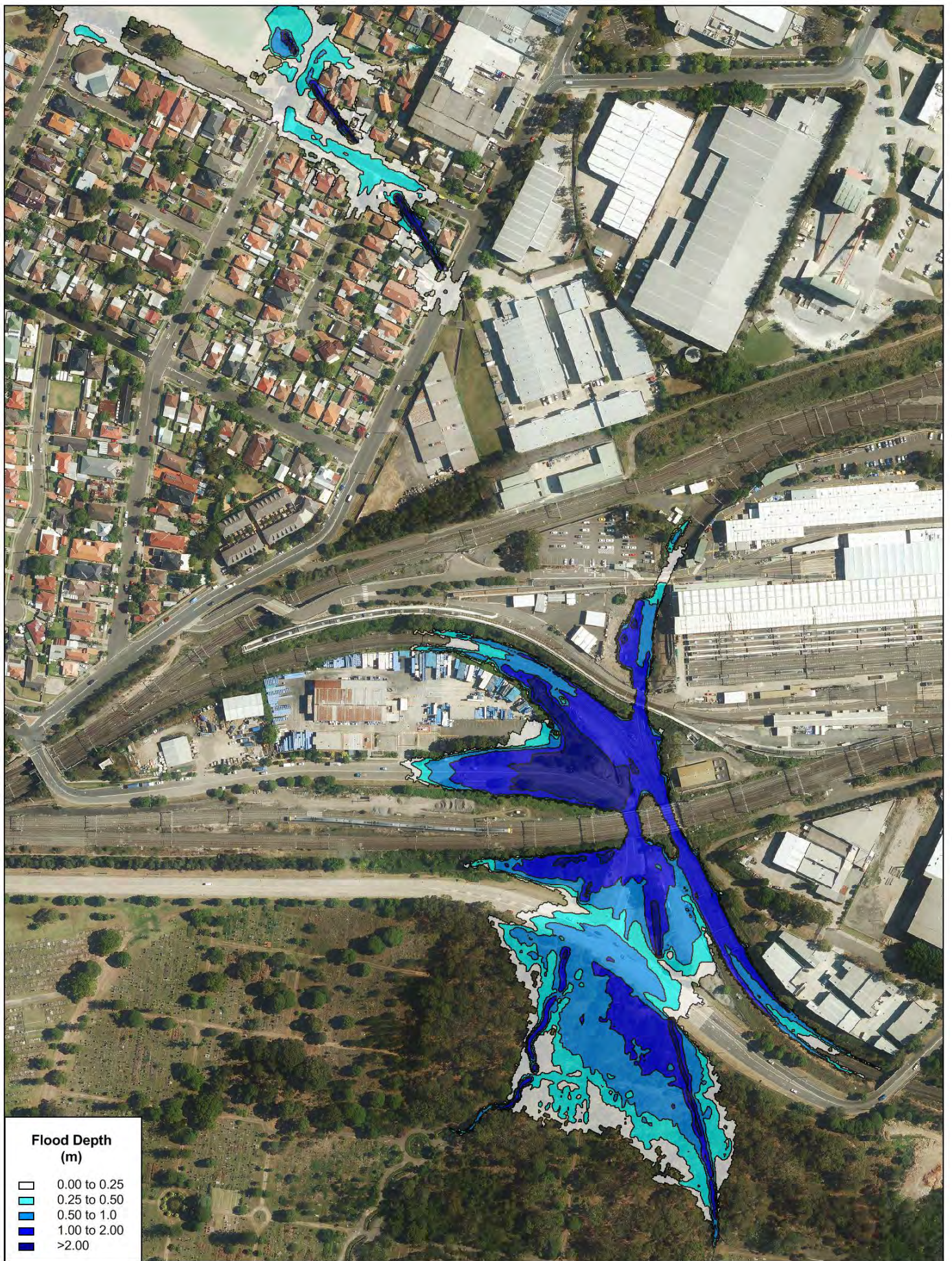
FIGURE C3 Design Scenario - 1% AEP + Climate Change Flood Depths
