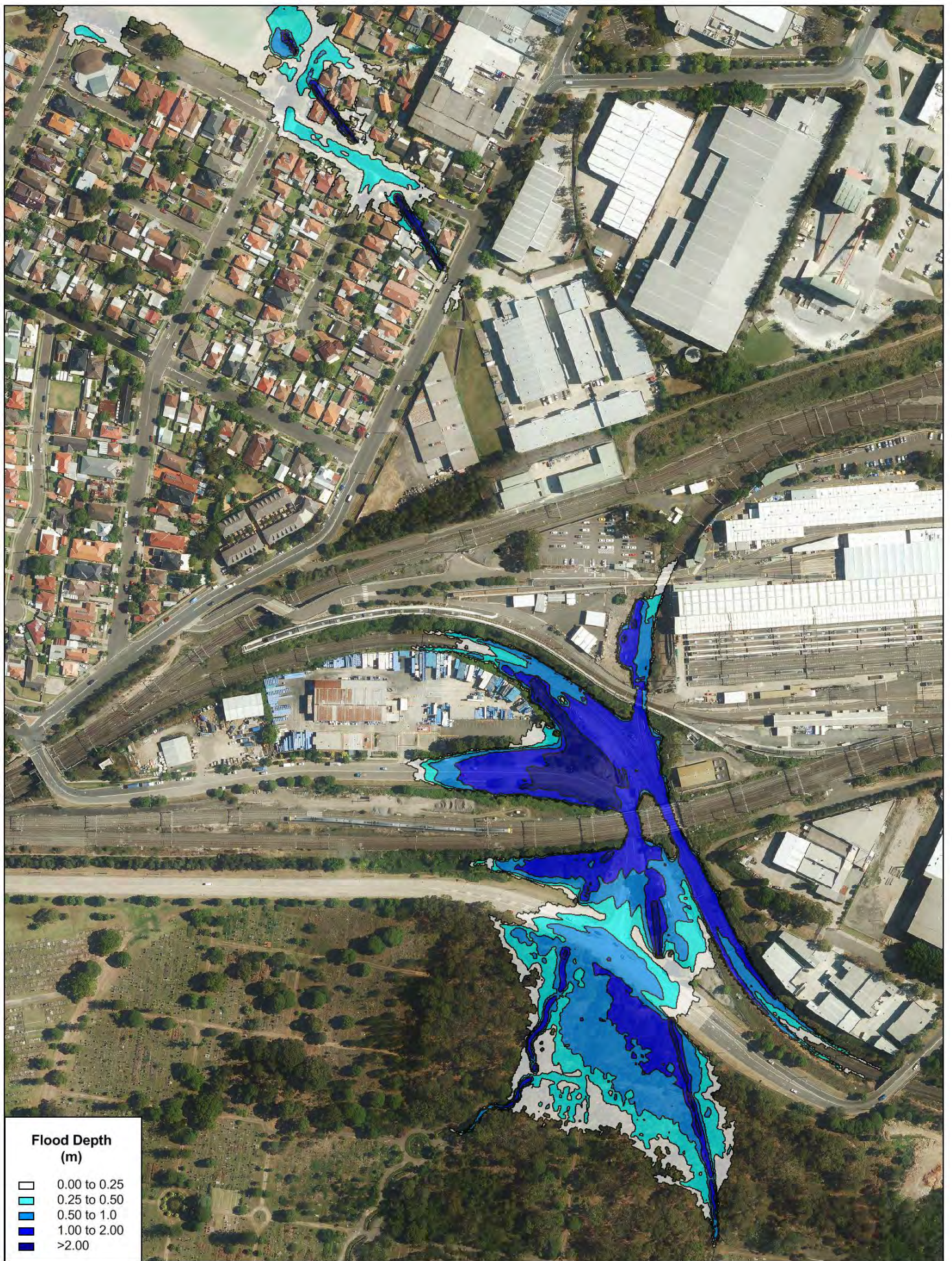
FIGURE C2 Design Scenario - 1% AEP Flood Depths
