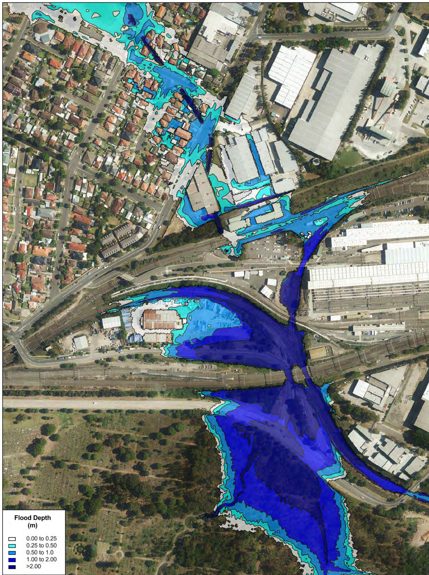
FIGURE B4 Existing Scenario - PMF Flood Depths
